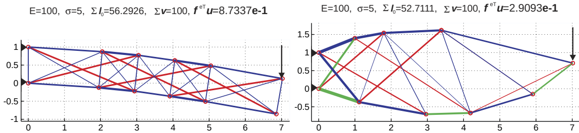
Fig. 2. Initial vs. optimized tensegrity beam design in loaded state, showing deformation under load. Legend: green (light gray)—slack strings, red (dark gray)—compressed bars, black (blue)—stretched strings. (For interpretation of the references in colour in this figure legend, the reader is referred to the web version of this article.)
